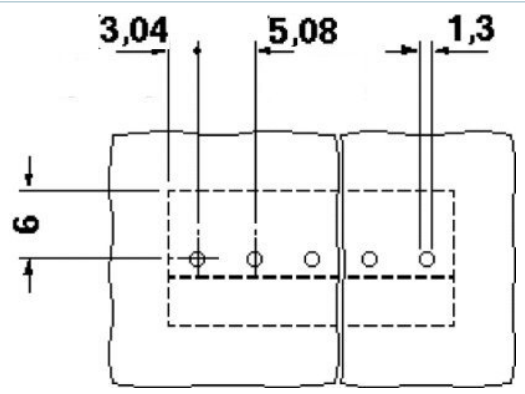
Dimensioned drawing
